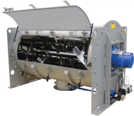
Batch-Type Single Shaft Mixers
