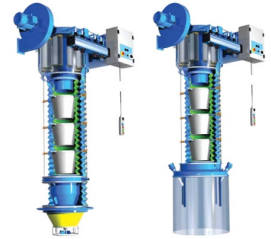
Loading Bellow
